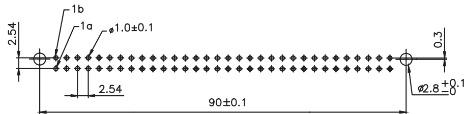
PCB Layout
